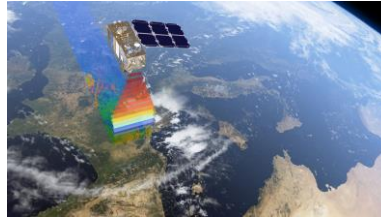
EARTH OBSERVATION
